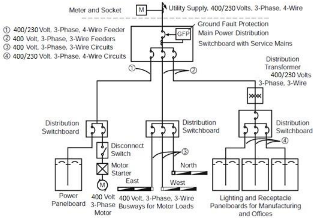
Switchboard
