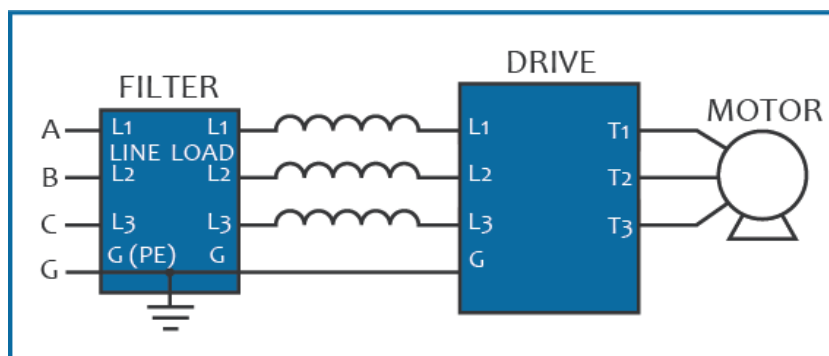
RFI filter
