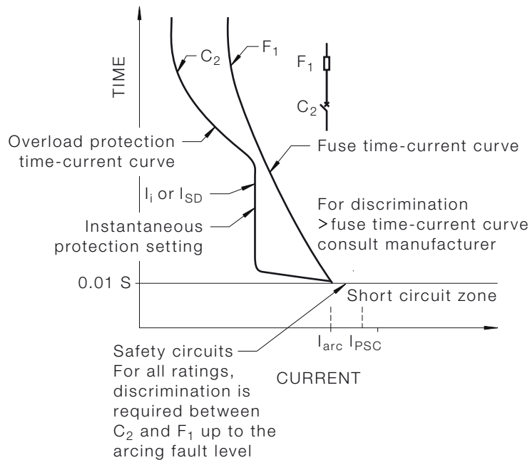
FIGURE 2.14 FUSE AND CIRCUIT-BREAKER CURVES WITH DISCRIMINATION REQUIREMENTS
