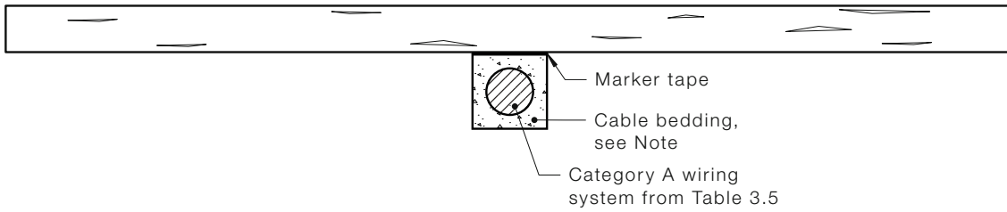
FIGURE 3.12 EXAMPLE OF A CATEGORY A UNDERGROUND WIRING SYSTEM WITH CABLE LOCATED DIRECTLY BELOW POURED CONCRETE OF 75 MM MINIMUM THICKNESS WITHIN THE CONFINES OF A BUILDING
