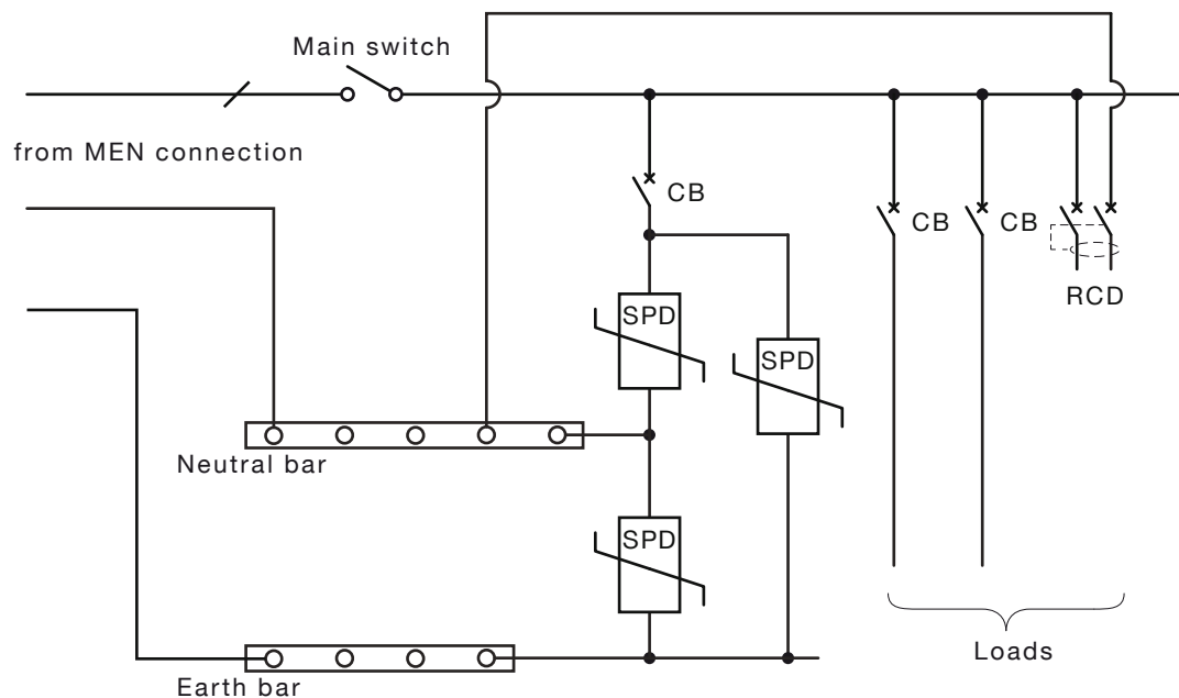
FIGURE F1.2 SECONDARY SPD ON DISTRIBUTION BOARD
