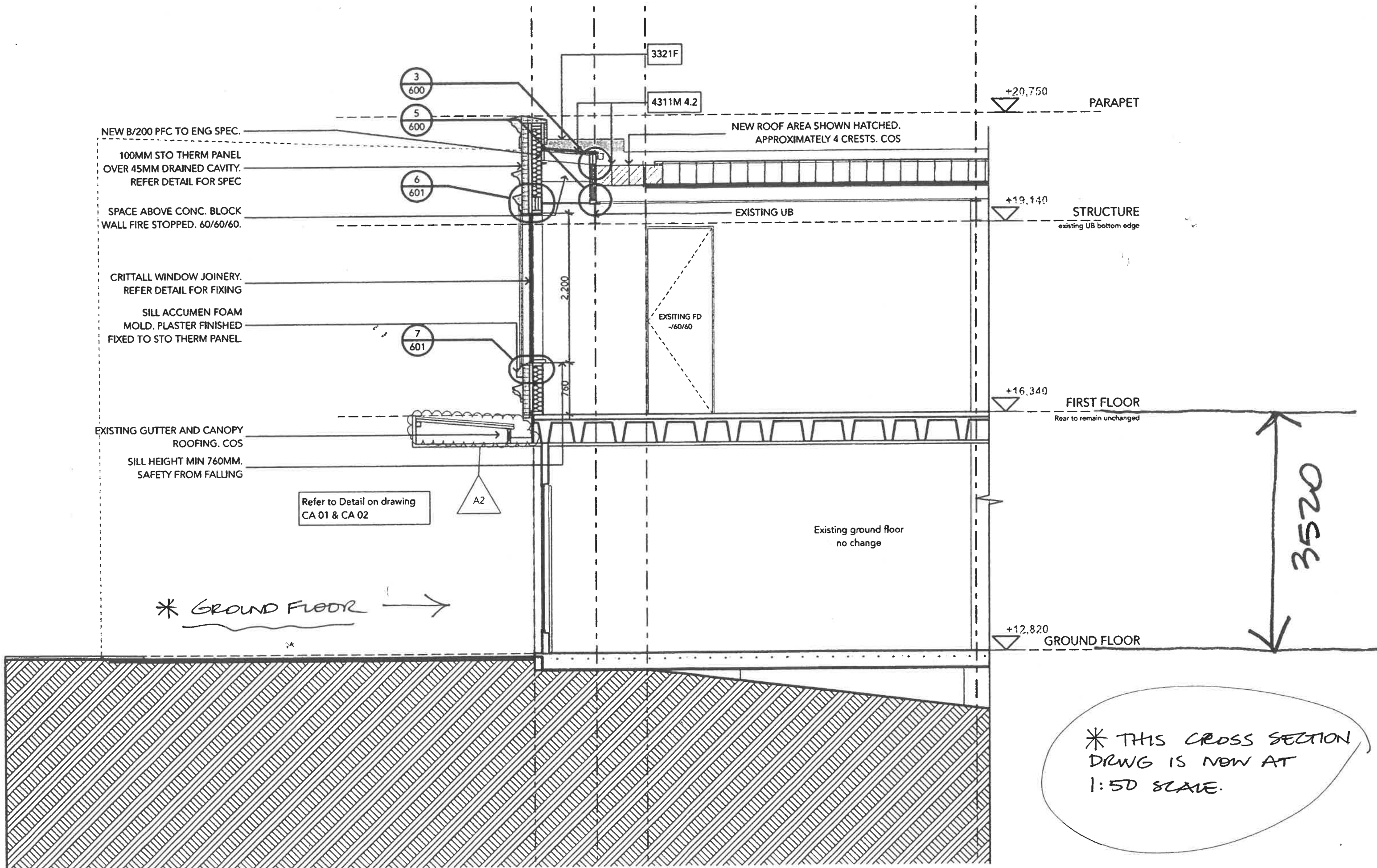
1 Section BB 501 Scale 1:50
