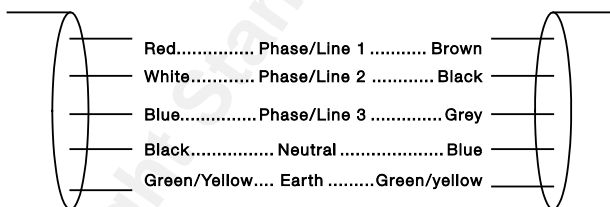
FIGURE 3.2 MULTI-PHASE CABLES
