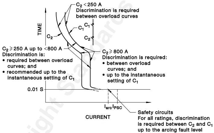
FIGURE 2.12 CIRCUIT-BREAKER CURVES WITH DISCRIMINATION REQUIREMENTS
