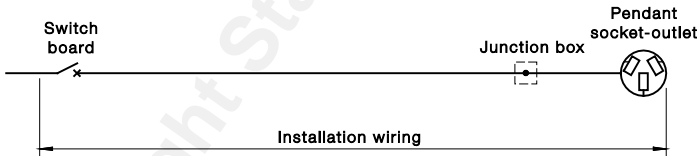
FIGURE 4.6 EQUIPMENT WIRING—EXCEPTION FOR PENDANT SOCKET-OUTLET
