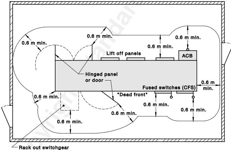
FIGURE 2.15 ACCESS TO SWITCHBOARDS—FREESTANDING SWITCHBOARD WITH RACK-OUT SWITCHGEAR
