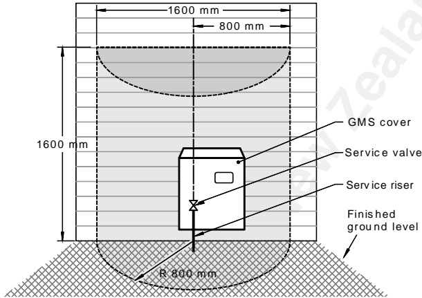
FIGURE 4.11 HAZARDOUS AREA FOR RETICULATED GAS SUPPLY REGULATORS
