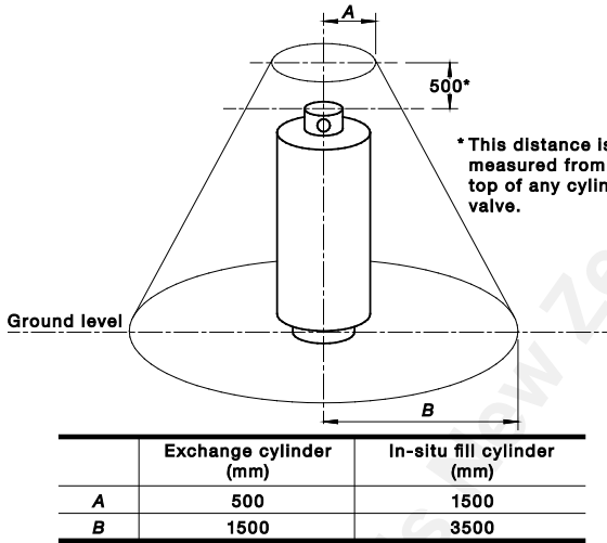
FIGURE 4.10 HAZARDOUS AREA PRESENTED BY A GAS CYLINDER OUTDOORS FOR HEAVIER-THAN-AIR GASES
