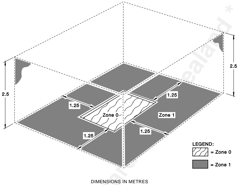
FIGURE 6.15 ZONE DIMENSIONS OF IN-GROUND SPA POOLS AND TUBS WITH WATER CAPACITY NOT EXCEEDING 5000 L
