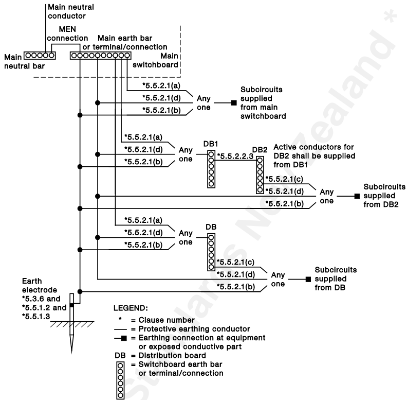
FIGURE 5.3 EXAMPLES OF EARTHING ARRANGEMENTS (CLAUSES 5.5.2.1 AND 5.5.2.3)
