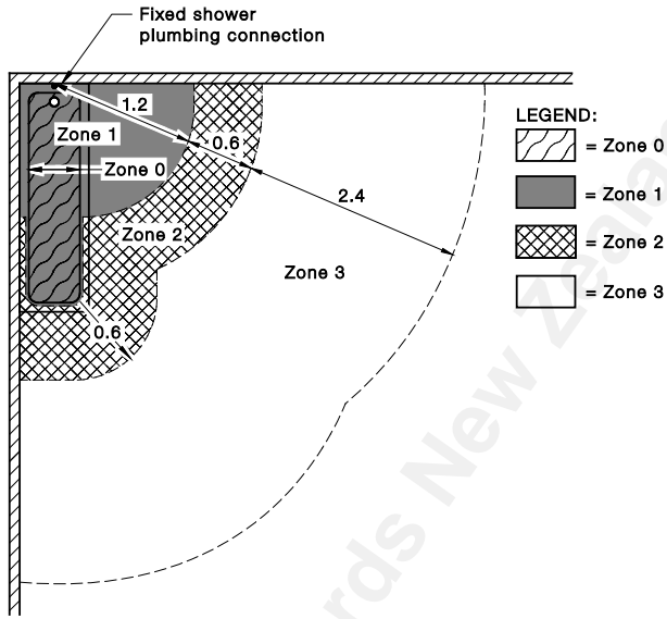
FIGURE 6.6 BATHS AND SHOWERS, ZONE DIMENSIONS (PLAN)—BATH WITH SHOWER WITHOUT BARRIER
