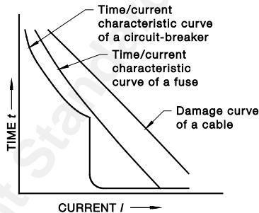
FIGURE B2 TYPICAL OVERCURRENT PROTECTION OF CONDUCTORS
