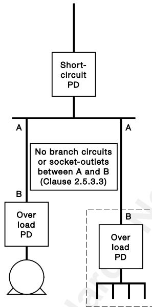
FIGURE 2.3 CLAUSE 2.5.3.3 (a)—ALTERNATIVE POSITION OF OVERLOAD PROTECTIVE DEVICE
