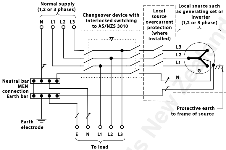
FIGURE 7.2 EXAMPLE OF CONNECTION OF AN ALTERNATIVE SUPPLY TO A SWITCHBOARD WITH A LOCAL MEN CONNECTION (THREE POLE/FOUR POLE CHANGEOVER)
