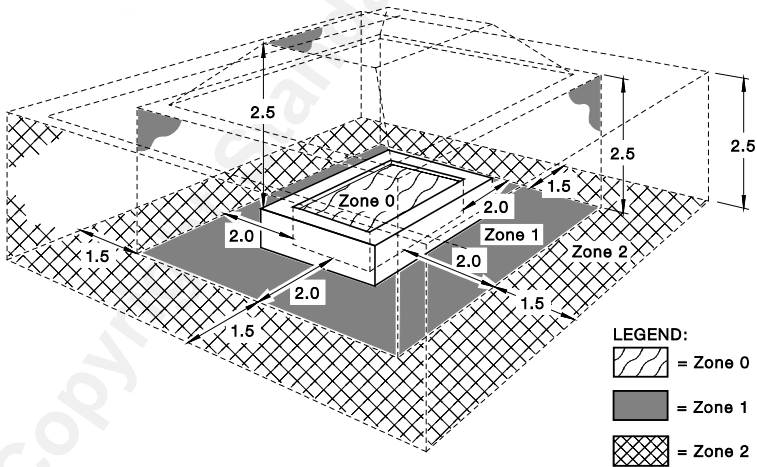
FIGURE 6.13 ZONE DIMENSIONS OF ABOVE-GROUND SWIMMING POOLS
