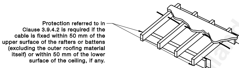
FIGURE 3.7 PROTECTION OF WIRING BELOW ROOFING MATERIAL
