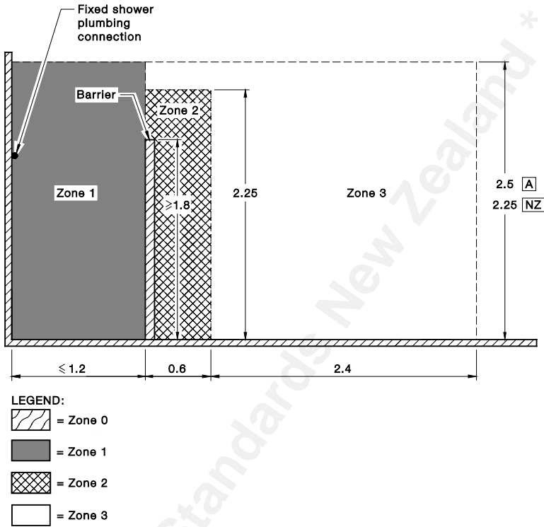
FIGURE 6.8 BATHS AND SHOWERS, ZONE DIMENSIONS (ELEVATION)— SHOWER WITH BARRIER
