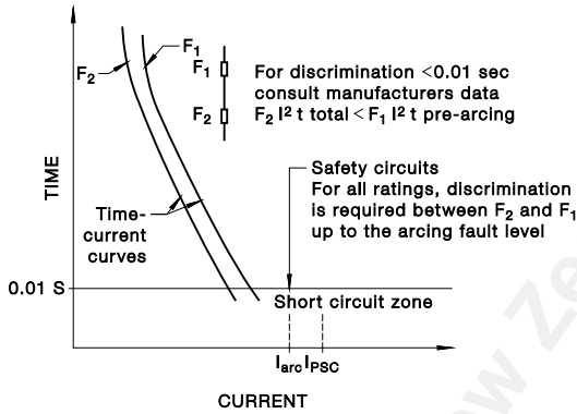
FIGURE 2.13 FUSE CURVES WITH DISCRIMINATION REQUIREMENTS
