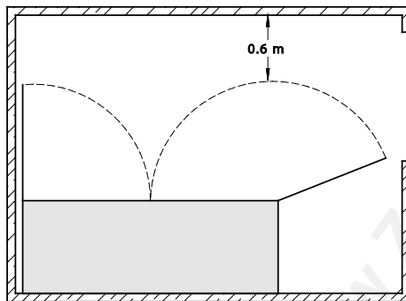
FIGURE 2.16 ACCESS TO SWITCHBOARDS— SWITCHBOARD IN CORNER POSITION
