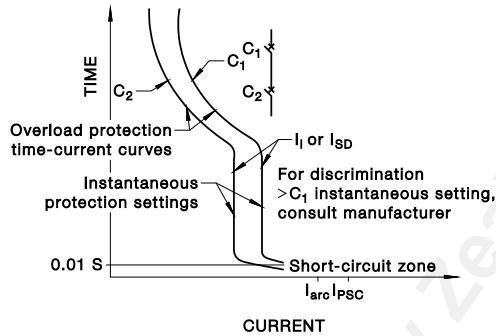
FIGURE 2.11 CIRCUIT-BREAKER CURVES—GENERAL EXPLANATION, SETTINGS AND ZONES
