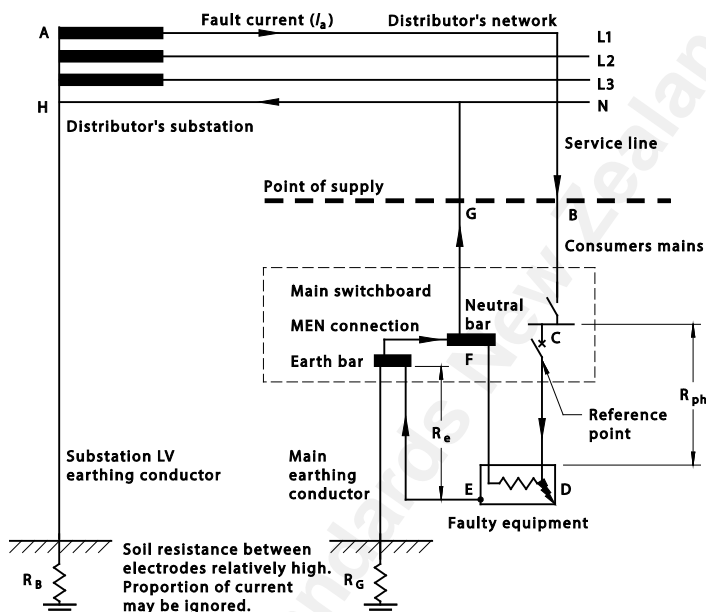
FIGURE B5 MEN SYSTEM (SIMPLIFIED)—SHOWING FAULT CURRENT ( I_a ) PATH (EARTH FAULT-LOOP)
