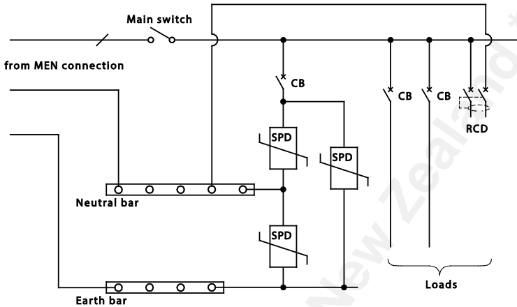
FIGURE F1.2 SECONDARY SPD ON DISTRIBUTION BOARD
