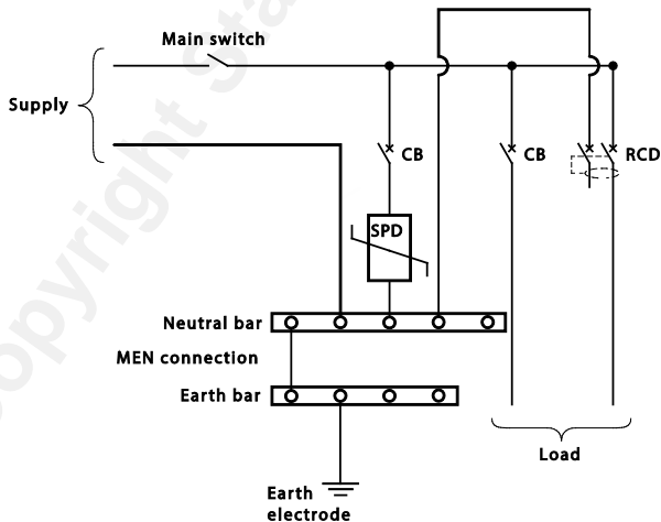
FIGURE F1.1 PRIMARY SPD ON MAIN SWITCHBOARD
