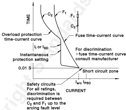
FIGURE 2.14 FUSE AND CIRCUIT-BREAKER CURVES WITH DISCRIMINATION REQUIREMENTS
