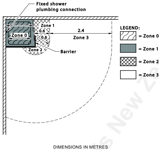
FIGURE 6.7 BATHS AND SHOWERS, ZONE DIMENSIONS (PLAN)—ENCLOSED SHOWER
