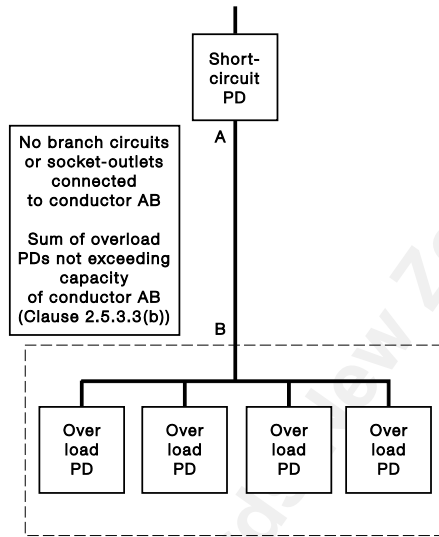
FIGURE 2.4 CLAUSE 2.5.3.3(b)—ALTERNATIVE POSITION OF OVERLOAD PROTECTIVE DEVICE
