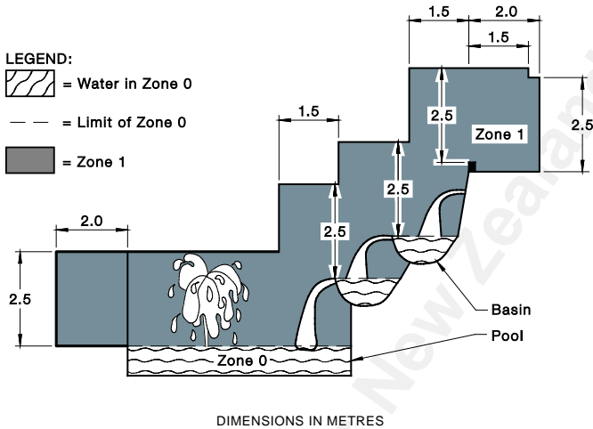
FIGURE 6.18 EXAMPLE OF DETERMINATION OF THE ZONES OF A FOUNTAIN (ELEVATION)
