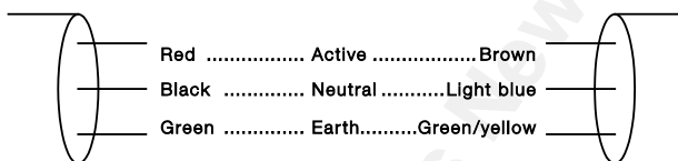
FIGURE 3.1 SINGLE-PHASE CABLES
