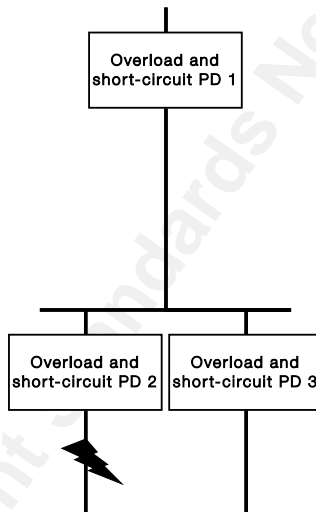
FIGURE 2.10 DISCRIMINATION BETWEEN PROTECTIVE DEVICES—GENERAL
