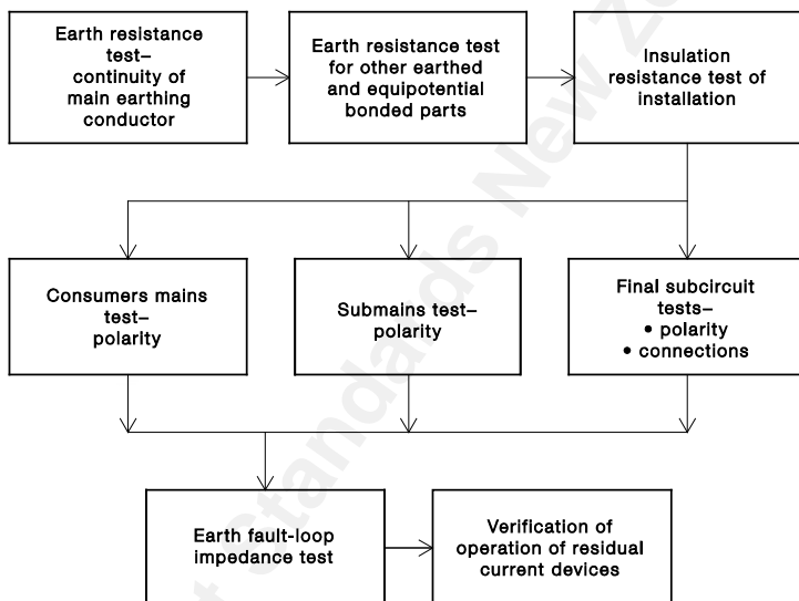
FIGURE 8.1 TESTING SEQUENCE
