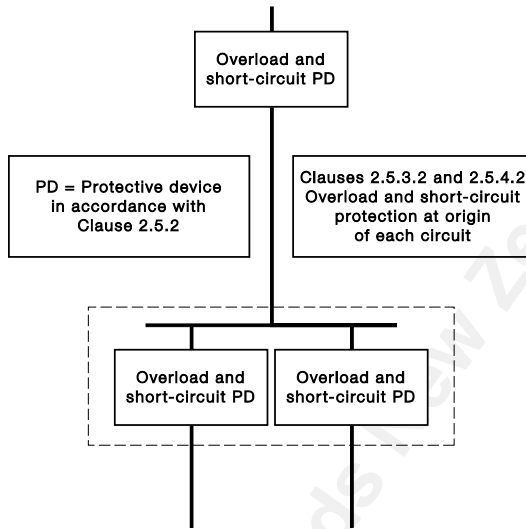
FIGURE 2.1 CLAUSES 2.5.1, 2.5.3.2 AND 2.5.4.2 GENERAL PROTECTION ARRANGEMENT
