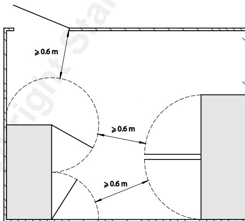
FIGURE 2.19 ACCESS TO SWITCHBOARDS— FACING SWITCHBOARDS
