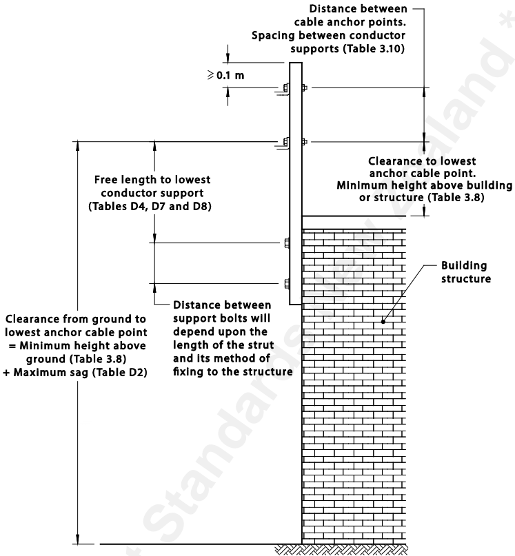
FIGURE D2 GUIDE TO SELECTION OF STRUTS
