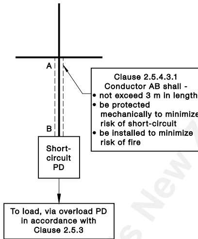
FIGURE 2.7 CLAUSE 2.5.4.3—ALTERNATIVE POSITION OF SHORT-CIRCUIT PROTECTIVE DEVICE
