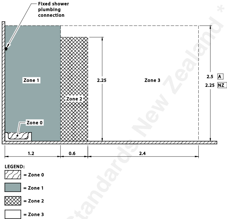
FIGURE 6.4 BATHS AND SHOWERS, ZONE DIMENSIONS (ELEVATION)— SHOWER WITH BASE WITHOUT BARRIERS
