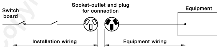
FIGURE 4.4 CONNECTION BY SOCKET-OUTLET
