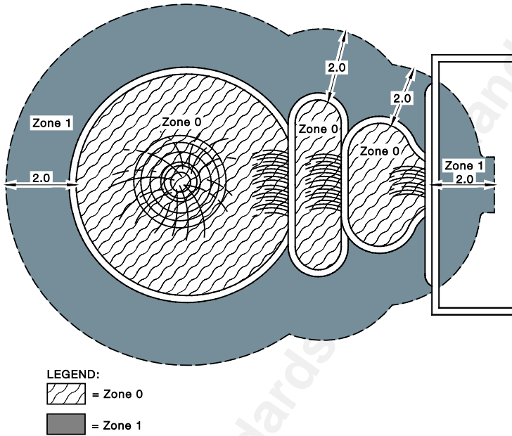
FIGURE 6.17 EXAMPLE OF DETERMINATION OF THE ZONES OF A FOUNTAIN (PLAN)
