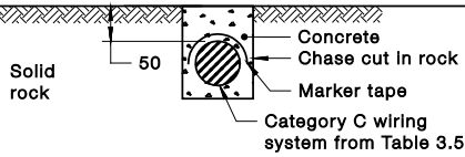
FIGURE 3.16 EXAMPLE OF A CATEGORY C UNDERGROUND WIRING SYSTEM
