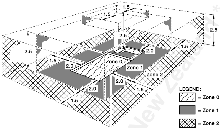
FIGURE 6.12 ZONE DIMENSIONS OF IN-GROUND SWIMMING POOLS
