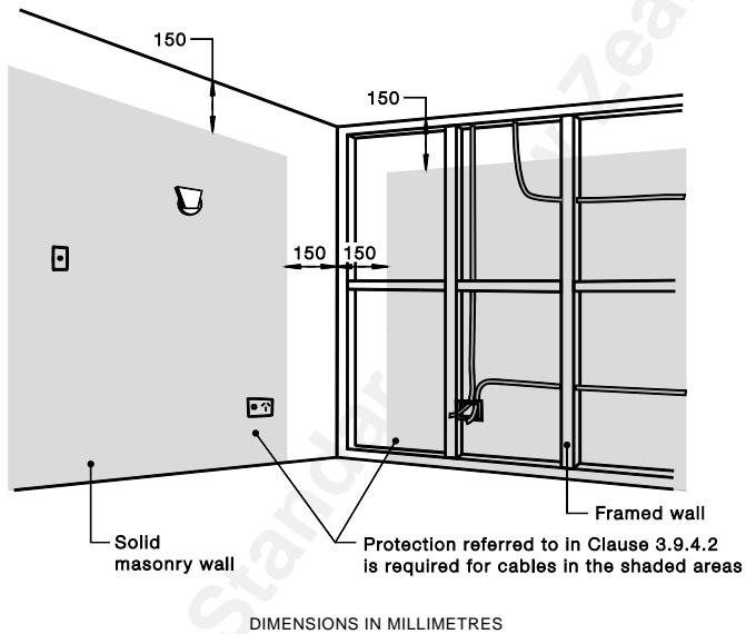
FIGURE 3.3 PROTECTION OF WIRING SYSTEMS WITHIN WALL SPACES
