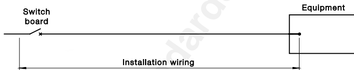
FIGURE 4.1 DIRECT CONNECTION
