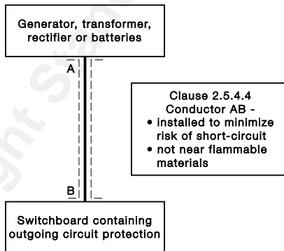
FIGURE 2.8 CLAUSE 2.5.4.4—OMISSION OF SHORT-CIRCUIT PROTECTION
