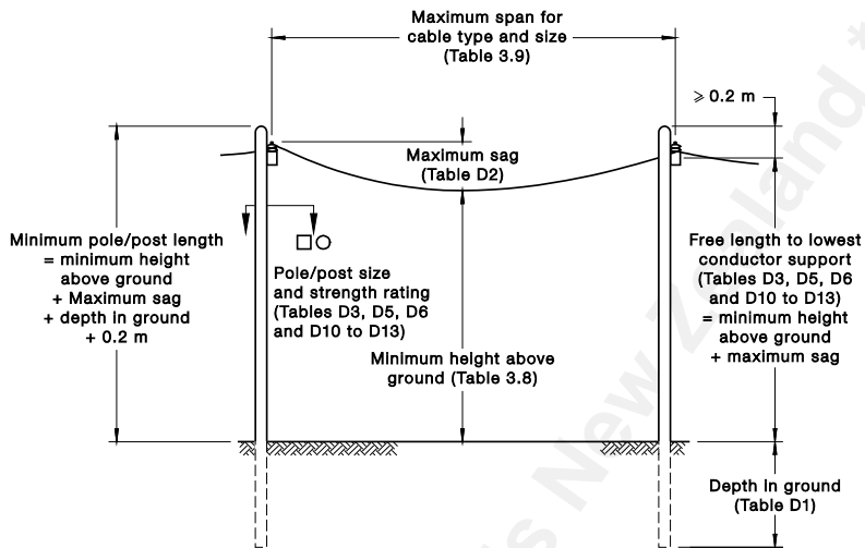
FIGURE D1 GUIDE TO SELECTION OF POLES/POSTS
