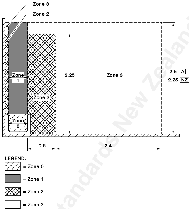
FIGURE 6.2 BATHS AND SHOWERS, ZONE DIMENSIONS (ELEVATION)— BATH WITHOUT SHOWER OR FIXED BARRIER
