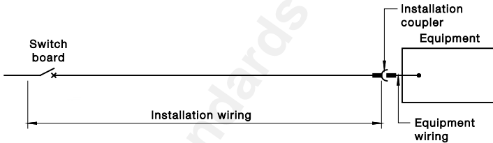
FIGURE 4.3 DIRECT CONNECTION BY INSTALLATION COUPLER-EXCEPTION
