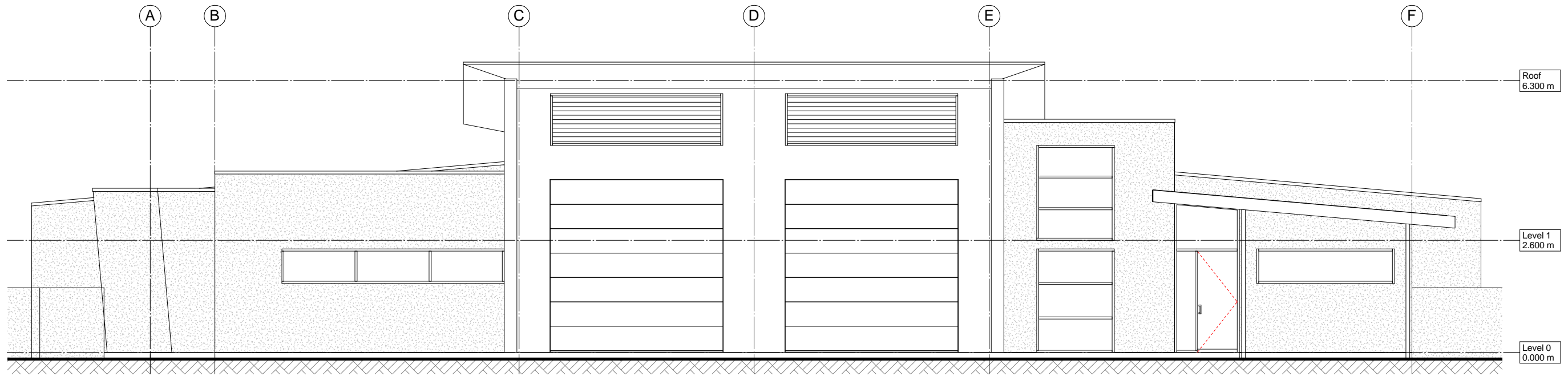
1 Elevation 1 - South A21 1:50
