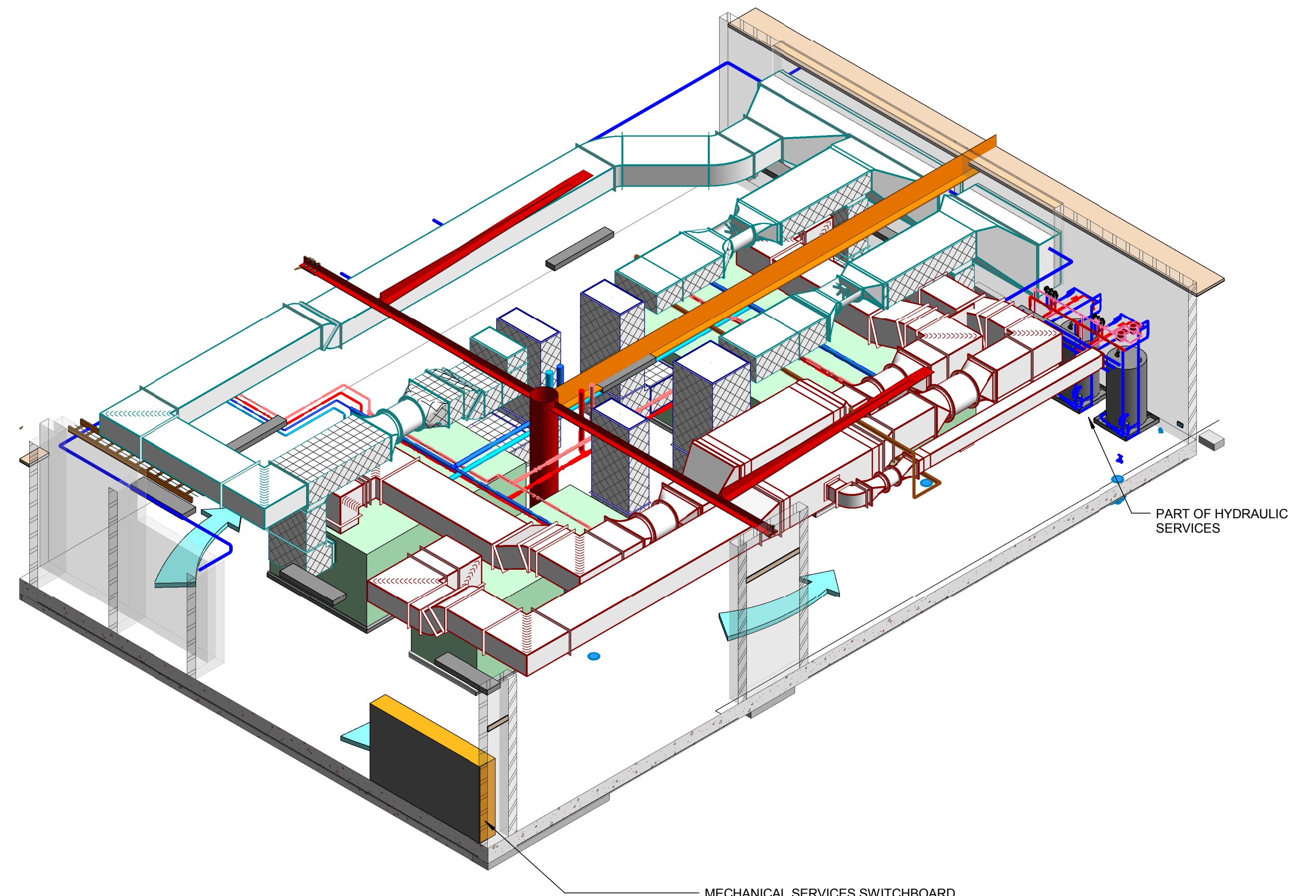
ISOMETRIC VIEW 2
