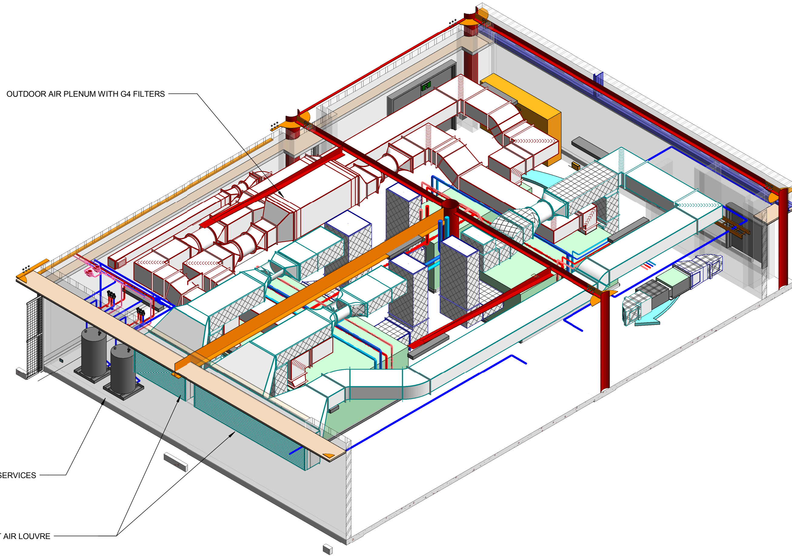
ISOMETRIC VIEW 1
